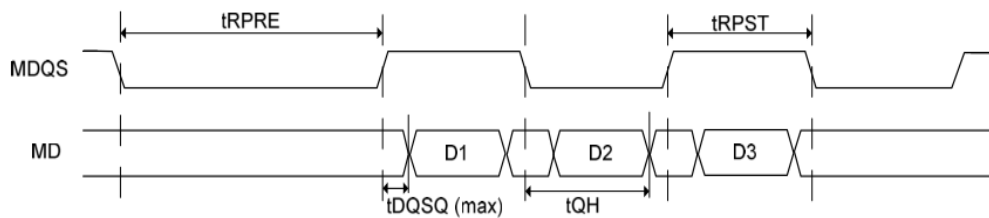
Figure 3-3 DDR2 SDRAM Read data
