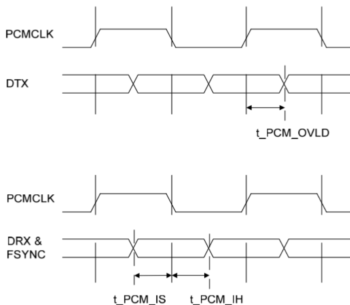
Figure 3-6 PCM Interface
