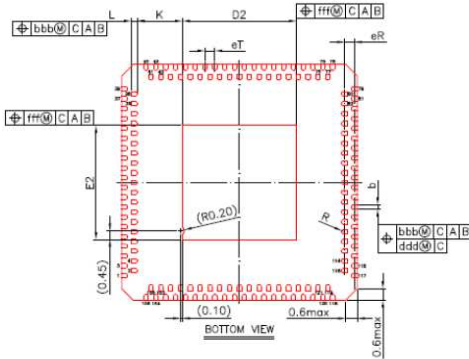
Figure 3-15 Bottom View
