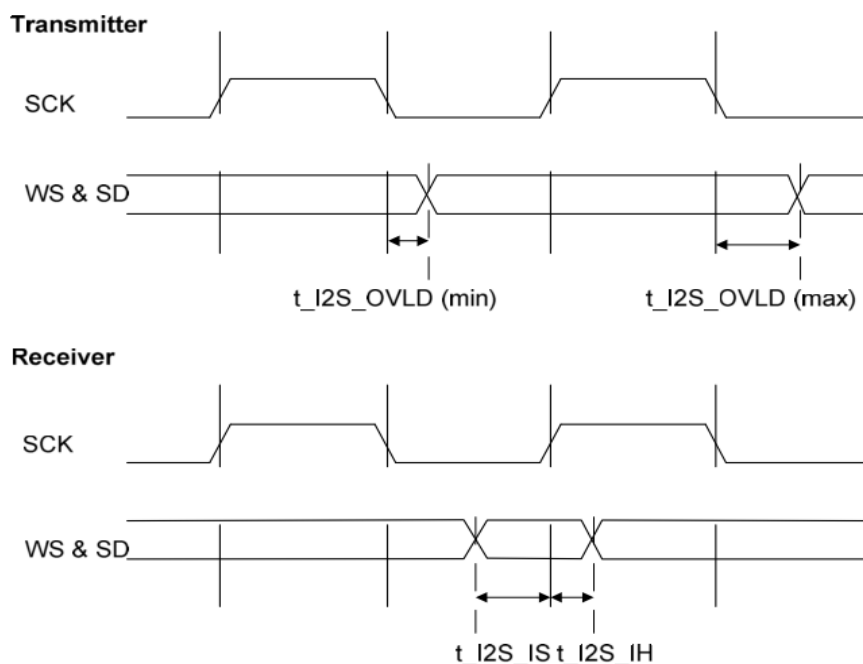
Figure-3-5 I2S Interface
