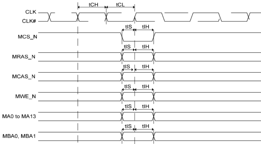
Figure 3-1 DDR2 SDRAM Command
