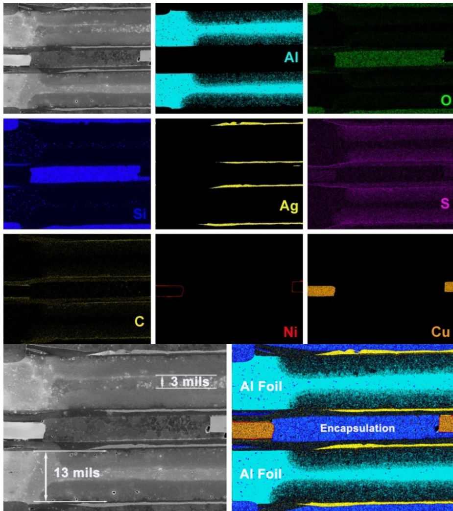
Figure 4. Two-dimensional EDX mapping results and cross-section SEM images of a 100 \mu\text{F} , 6V PA capacitor made by manufacturer E show a “laminated” structure.
