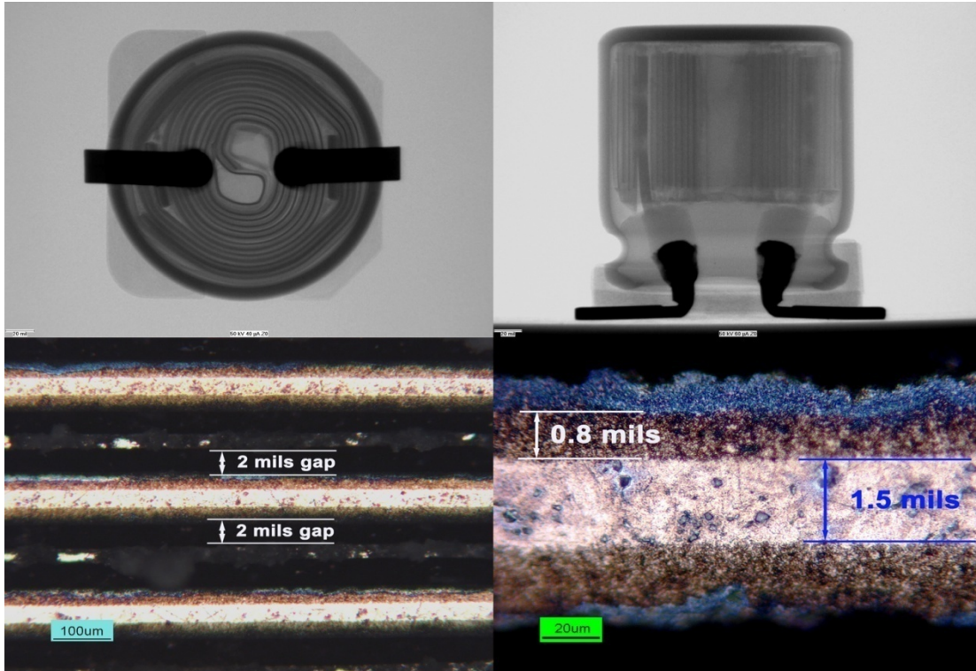
Figure 6. Radiographic images and high-magnification cross-sectional optical views of a 100 \mu\text{F} , 10 V PA capacitor made by manufacturer C show a traditional “wound” structure.
